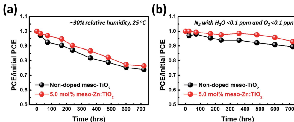
Fig. 9 Long-term stability of the PSCs with non-doped meso-TiO 2 and 5.0 mol% meso-Zn:TiO 2 (a) under the ambient atmosphere (~30% relative humidity, 25 °C) and (b) in the glovebox system (N 2 with H 2 O < 0.1 ppm and O 2 < 0.1 ppm).
