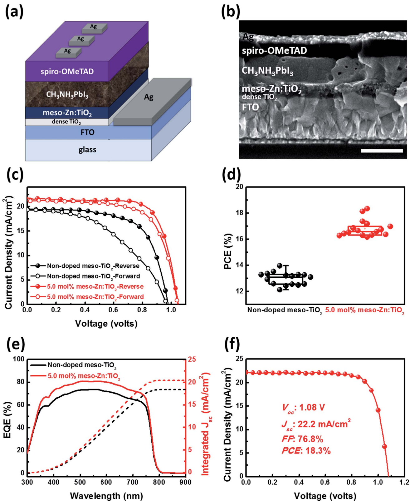
Fig. 8 (a) Schematic diagram and (b) cross-sectional SEM image of the PSC with 5.0 mol% meso-Zn:TiO 2 (scale bar = 500 nm). (c) J - V curves of the PSCs with non-doped meso-TiO 2 and 5.0 mol% meso-Zn:TiO 2 under reverse and forward scans. (d) PCE distribution and (e) EQE spectra of the PSCs with non-doped meso-TiO 2 and 5.0 mol% meso-Zn:TiO 2 . (f) J - V curve of the champion device.
