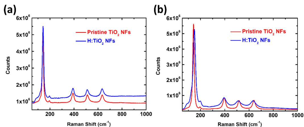
Figure 4. (a) 633 nm and (b) 532 nm excitation of TERS of pristine TiO 2 -650 NFs and H:TiO 2 -650 NFs.
