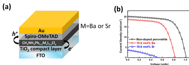
Fig. 4. (a) The schematic diagram of our perovskite solar cell structure. (b) J - V curves of the various perovskite solar cells, including non-doped perovskite solar cell, 10.0 mol% Sr-doped perovskite solar cell, and 10.0 mol% Ba-doped perovskite solar cell.
