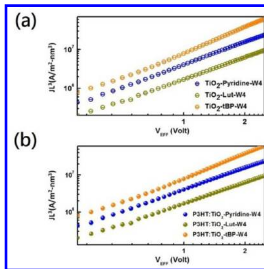
Figure 7. Electron mobility of different hybrid films determined by the space charge limited current model. (a) TiO 2 -(pyridine derivatives)-W4 thin film, and (b) P3HT:TiO 2 -(pyridine derivatives)-W4 hybrid thin film.
