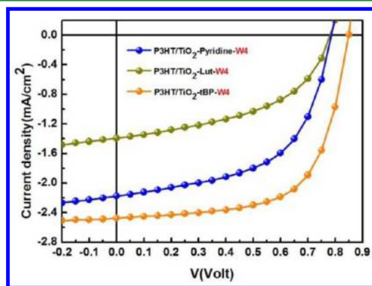
Figure 8. J-V curves of different P3HT:TiO 2 -(pyridine derivative)-W4 devices.
